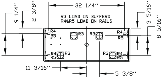
RAIL BRACKETS
