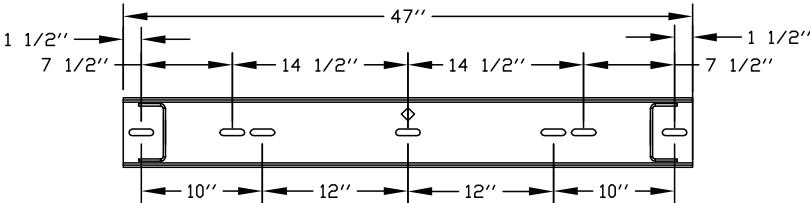
RAIL BRACKETS
